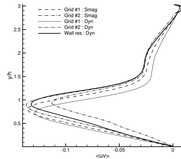
Figure 9: \langle uv \rangle at x/h = 2.0
