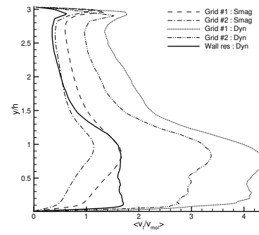
Figure 11: \langle \nu_t \rangle / \nu at x/h = 2.0
