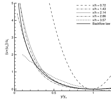
Figure 13: 'Backflow' scaling
