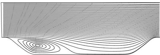
Figure 3: Typical mean streamlines
