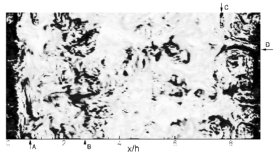
Figure 4: Near-wall vorticity
