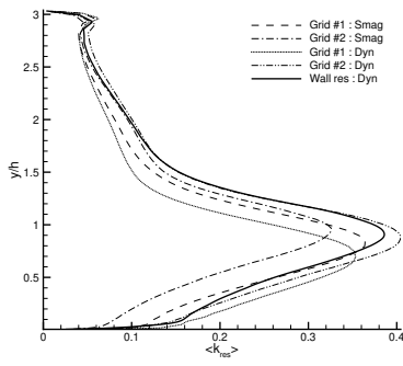
Figure 10: \langle k_{res} \rangle at x/h = 2.0
