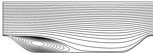
Figure 5: Streamlines for the highly-resolved simulation.
