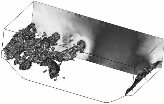
Figure 1: Constricted channel geometry with instantaneous pressure isosurfaces.
